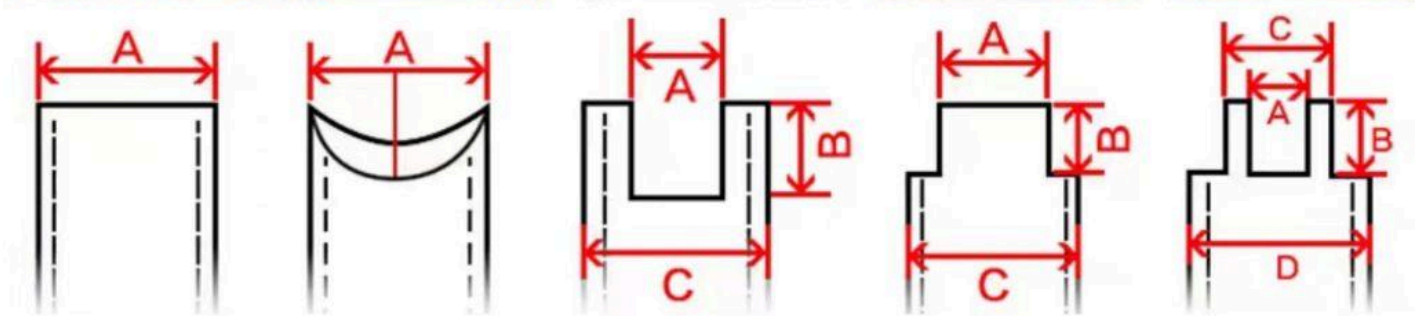
Flat end
